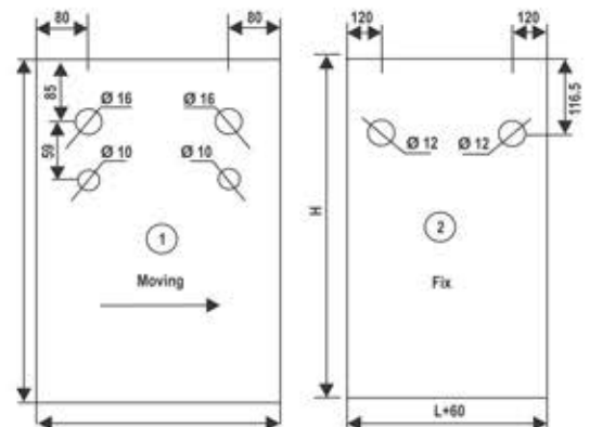
KZSL-11-A6 Track to Track Connector 90°
