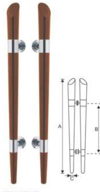
KZDH-WSS-77
