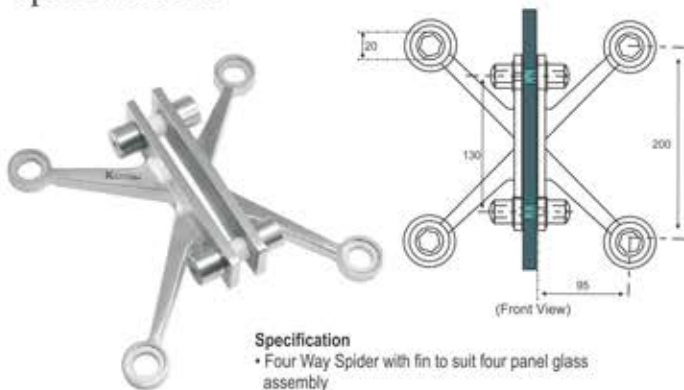
KZSP-A4 Four Way Spider
