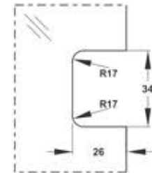
KZPF-640 Wall to Glass Connecting Patch
