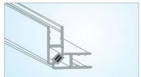
KZPS-M3 90° For : 8/10/12mm Glass Size : 2.2mtr / 2.5mtr
