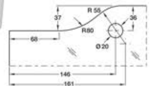
KZPL-2B Centre Lock Strike Box
