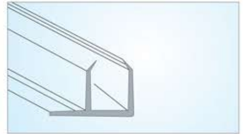
KZPS-06 For : 8/10/12mm Glass Size : 2.2mtr / 2.5mtr
