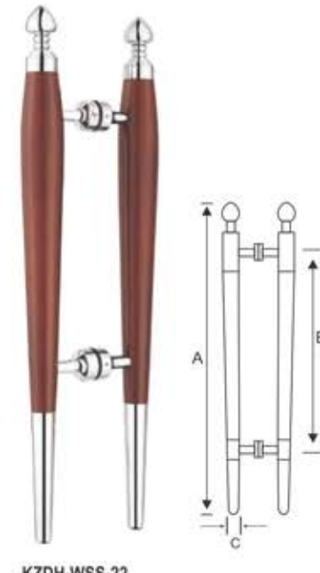
KZDH-WSS-22
