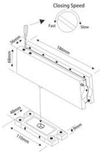
KZHFS-100 Hydraulic Floor Spring
