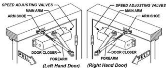
KZDC-3 Door Closer (with Pelmet Arm) Specification • Applicable Door Weight up to 90 kg. • Finish : Aluminium and SS
