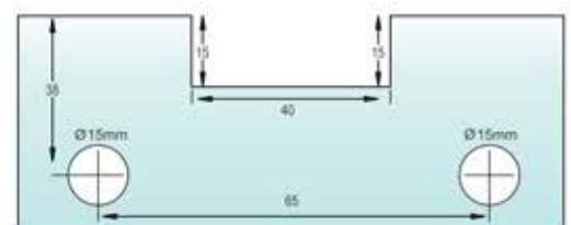
CUTOUT DETAILS OF CSL-44-R8
